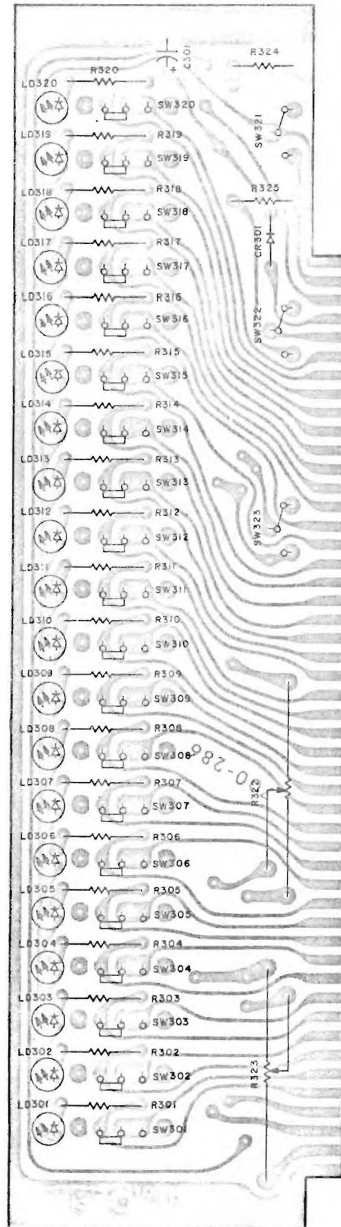
3-2 SWITCH BOARD PARTS PLACEMENT DIAGRAM
